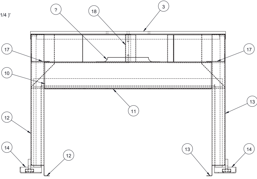
SECTION B-B
